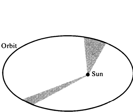
FIGURE 14.20. Kepler's second law. The two shaded regions, swept out in equal time intervals, have equal areas.
