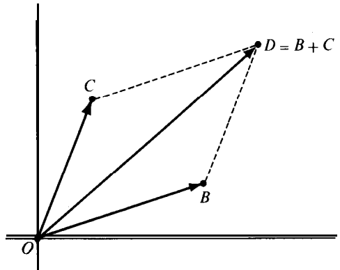
FIGURE 12.4 Vector addition interpreted geometrically by the parallelogram law.
