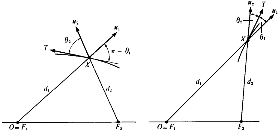
(a) \theta_2 = \pi - \theta_1 on the ellipse (b) \theta_2 = \theta_1 on the hyperbola
